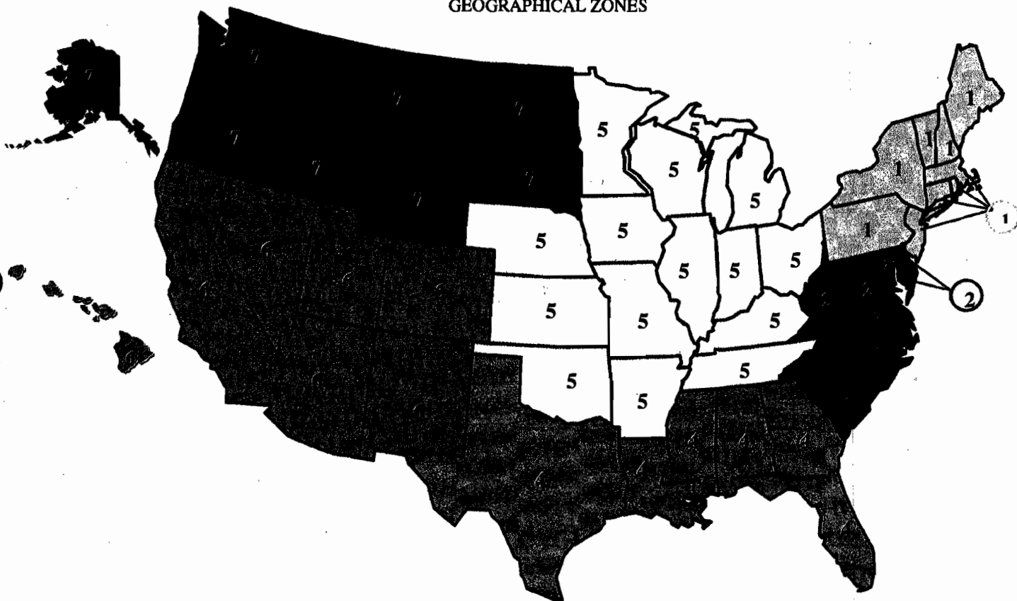
GEOGRAPHICAL ZONES
